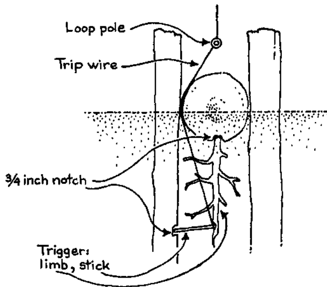
TWO POSSIBLE TRIGGER MECHANISMS
