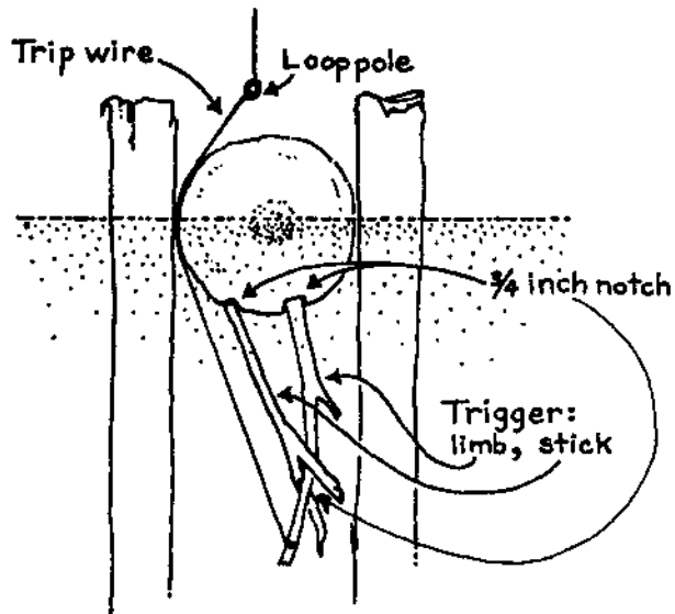
A Type Trigger
